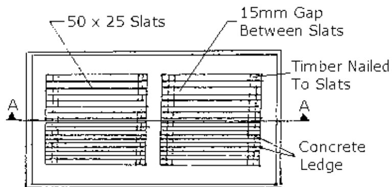
False Floor - Plan View
