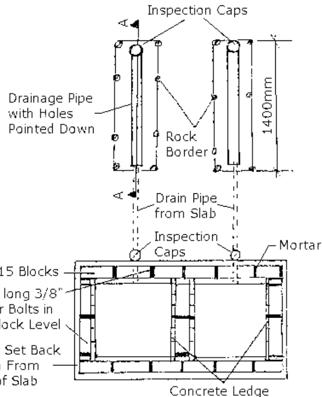
ET Bed Drainage Trenches - Plan View
